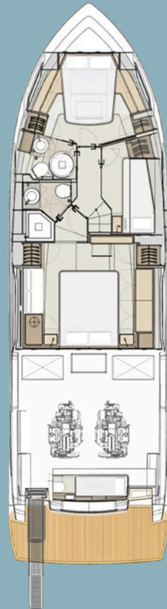
LOWER DECK
